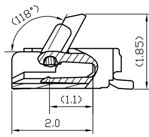
ACTUATOR OPEN STATE (SCALE 6:1)
